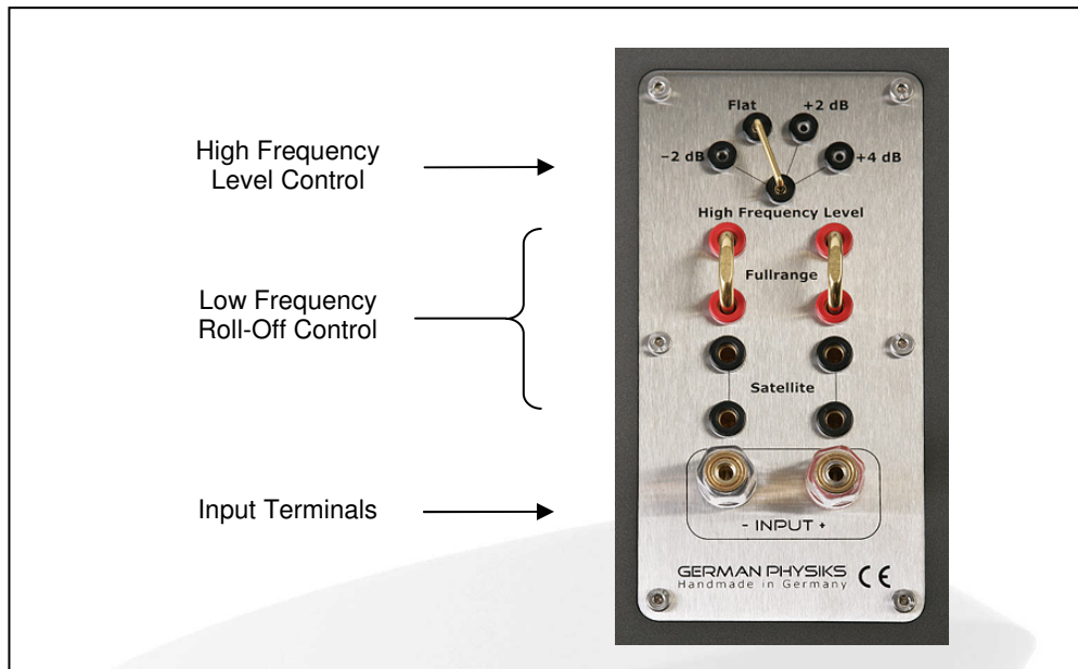
Figure 6. Input Terminals and Crossover Adjustments for Carbon Fibre DDD Troubadour 80
