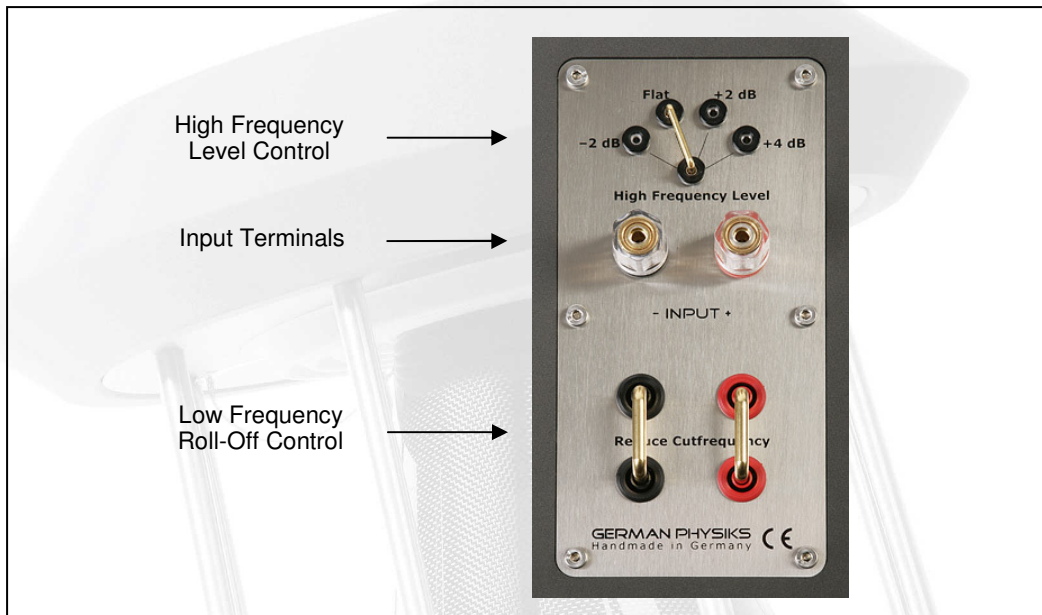
Figure 5. Input Terminals and Crossover Adjustments for Titanium DDD Troubadour 80
